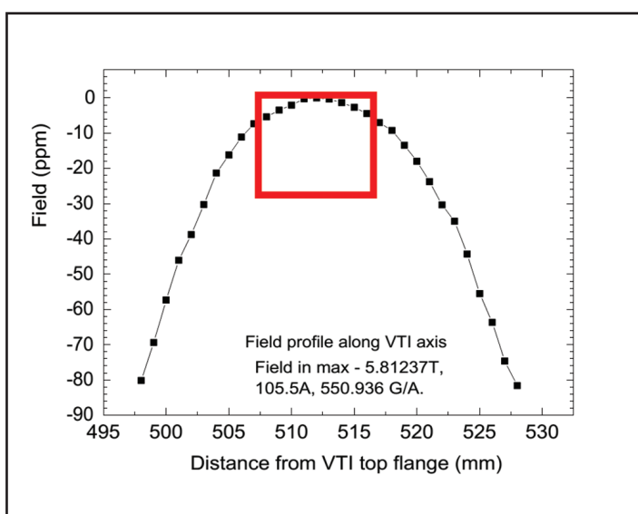
Field profile measured at low temperature and along the VTI
