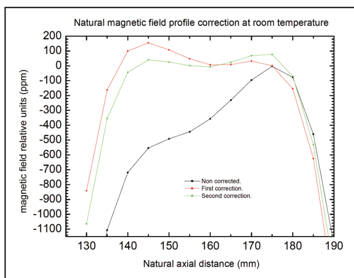
Once the magnet was cold the above results were measured at low temperature and along the VTI
